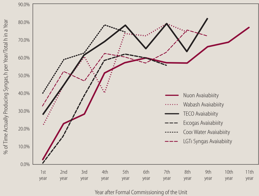
Figure A-3.B.13 History of IGCC Availability for the Start-up of Coal-based Units (excluding operation on back-up fuel)
