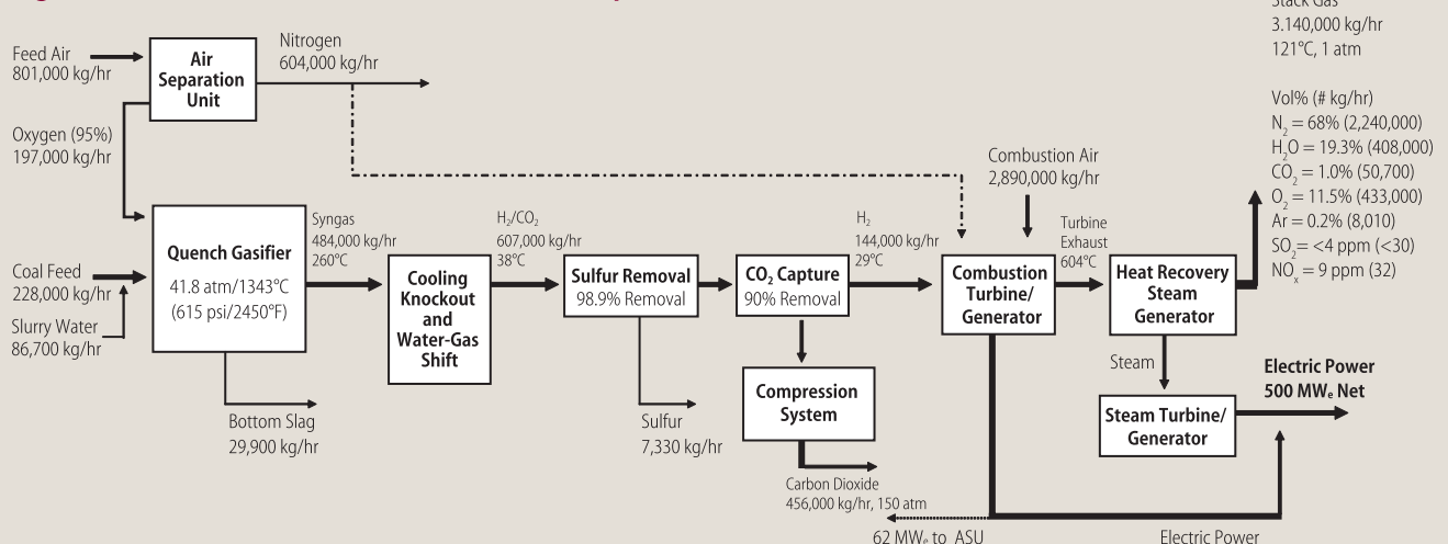
Figure A-3.B.12 500 MW e IGCC Unit with CO 2 Capture
